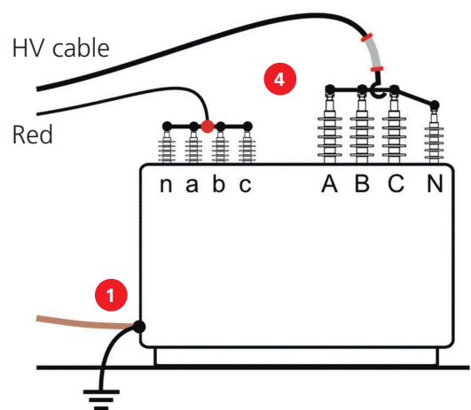
HV test connection for Delta / S1
