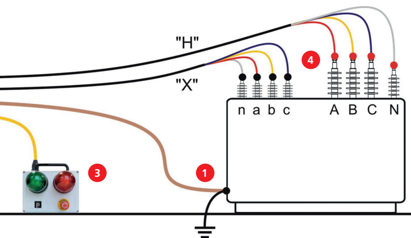
LV test connection for MTO / TTR
